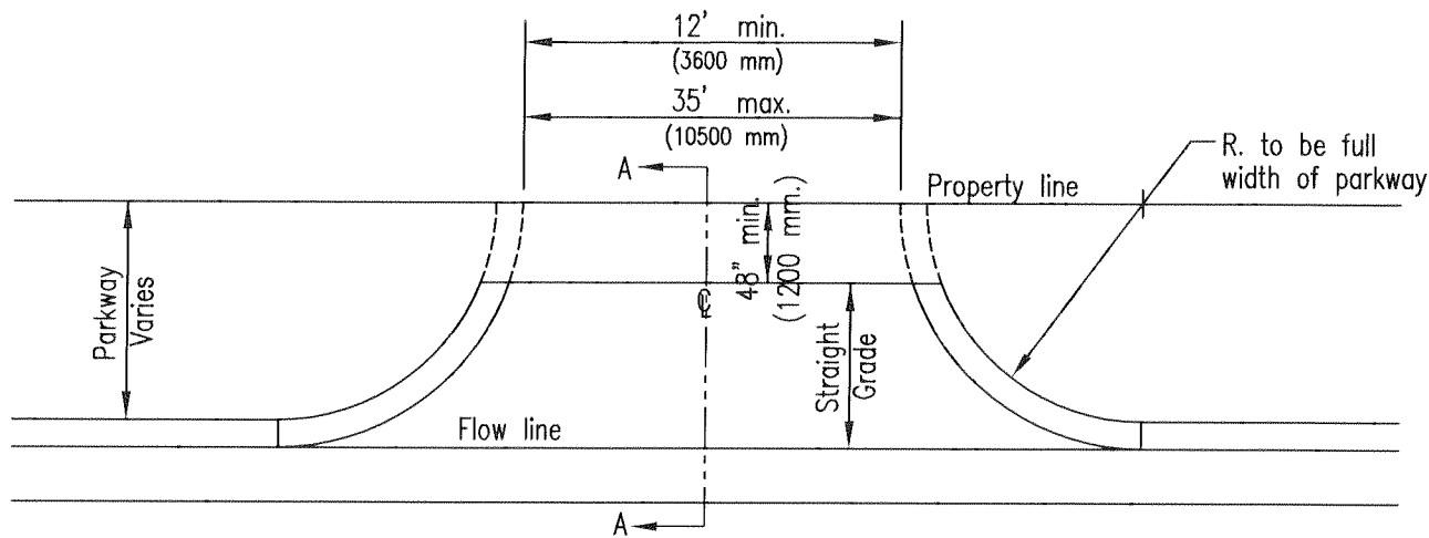
PLAN NTS
