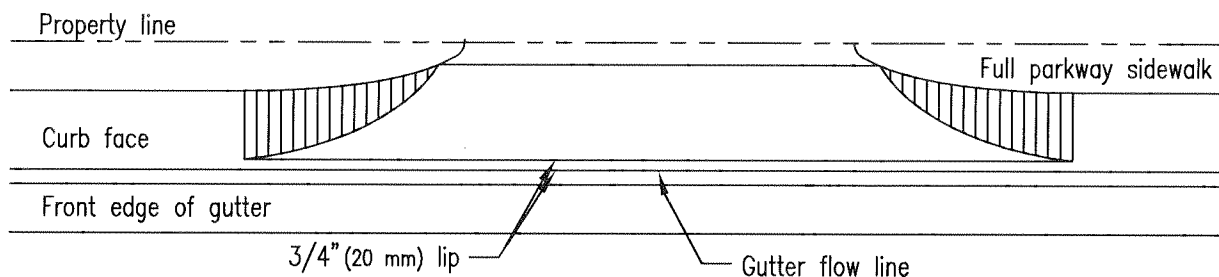
ELEVATION NTS
